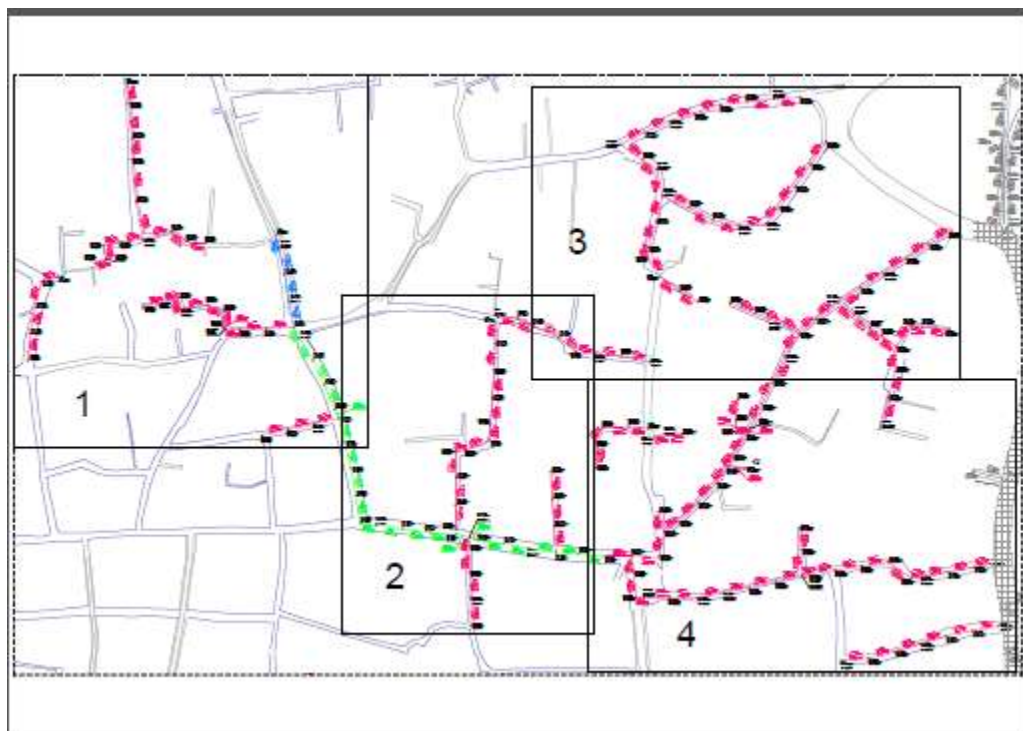
Figure 5-2 Laterals to be replaced in Zone III as a part of this DPR
